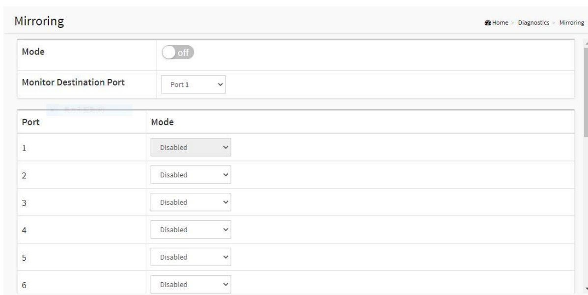
Figure 66: Mirroring
